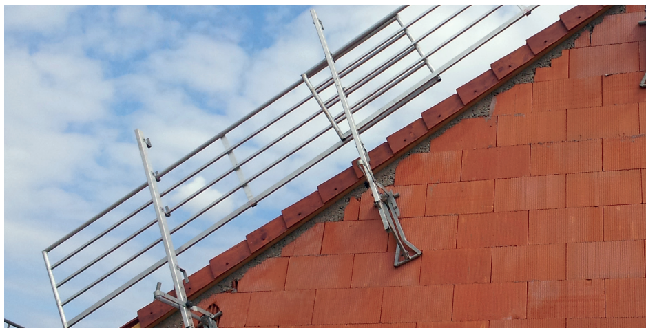
Potelet garde-corps polyvalent
